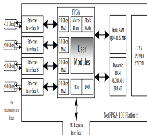
Fig. 1: NetFPGA-10G structure.
